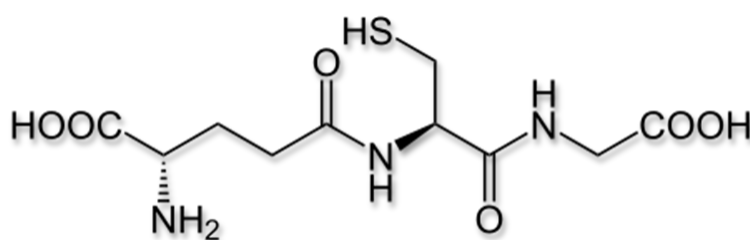
Reduced Glutathione(GSH)
